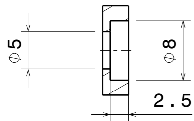
Section cut B-B
